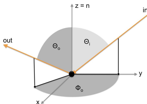
Figure 1: The geometry of the angles in a single BRDF measurement for the incoming light direction \mathbf{in} and outgoing light direction \mathbf{out} .
